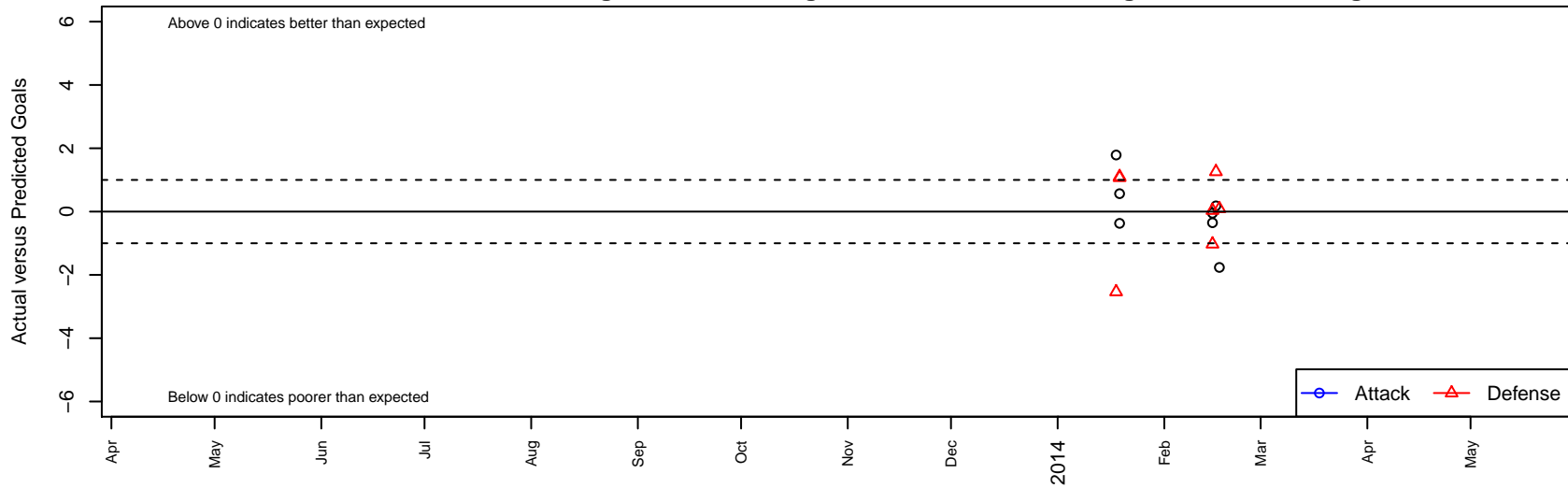
Forza FC Premier B99 Dots are actual minus expected GF (blue circles) and GA (red triangles). Blue line is smoothed change in attack strength. Red is smoothed change in defense strength.
